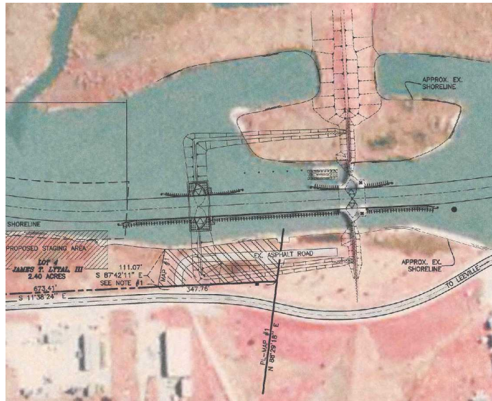
Distance between the two gates, which form the lock, is approximately 400 feet.
